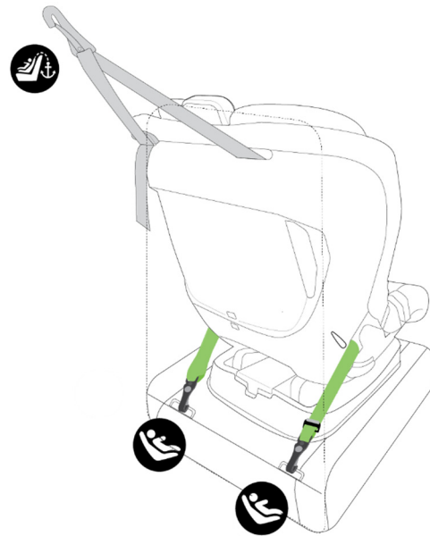
Forward-facing installation using lower anchors and tether
